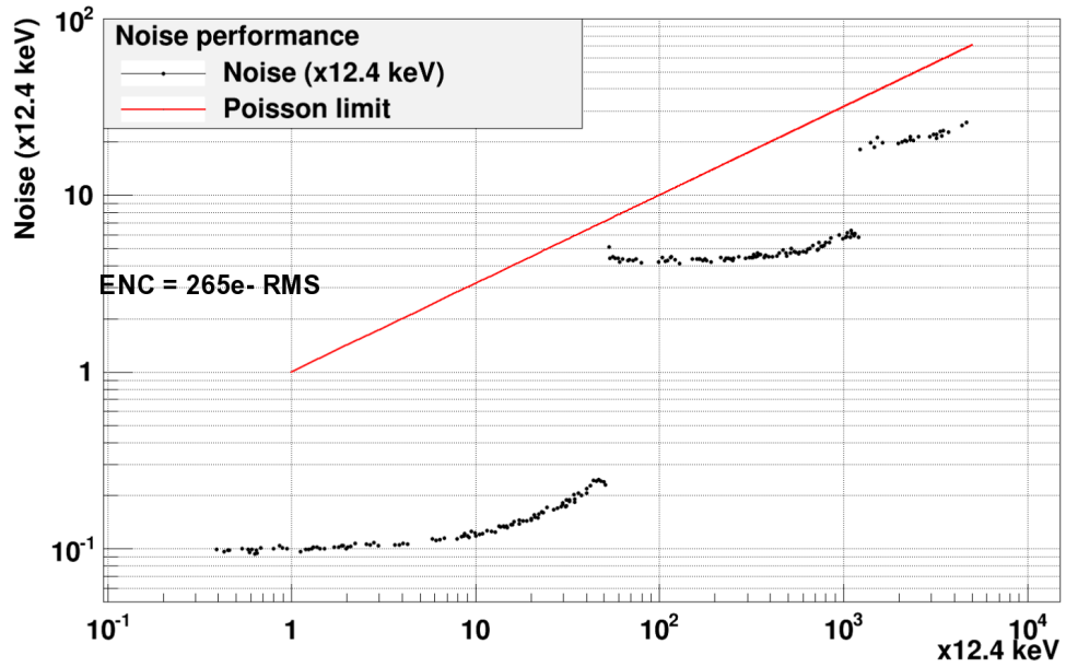
Figure 6. AGIPD 1.0 noise measurements.
