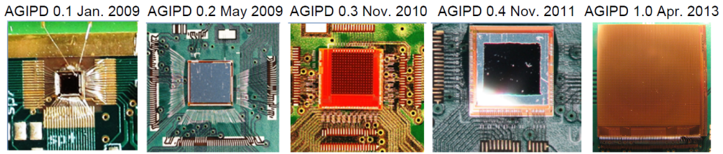
Figure 4. AGIPD runs prototypes and full scale ASIC.
